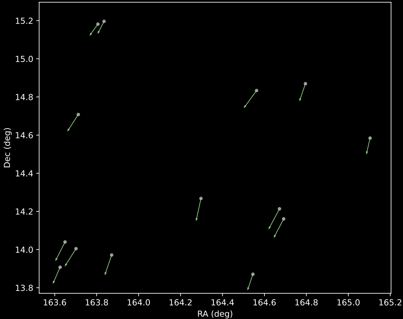
APOGEE DR17 Cluster 5 Proper Motion Vectors (n=14)
