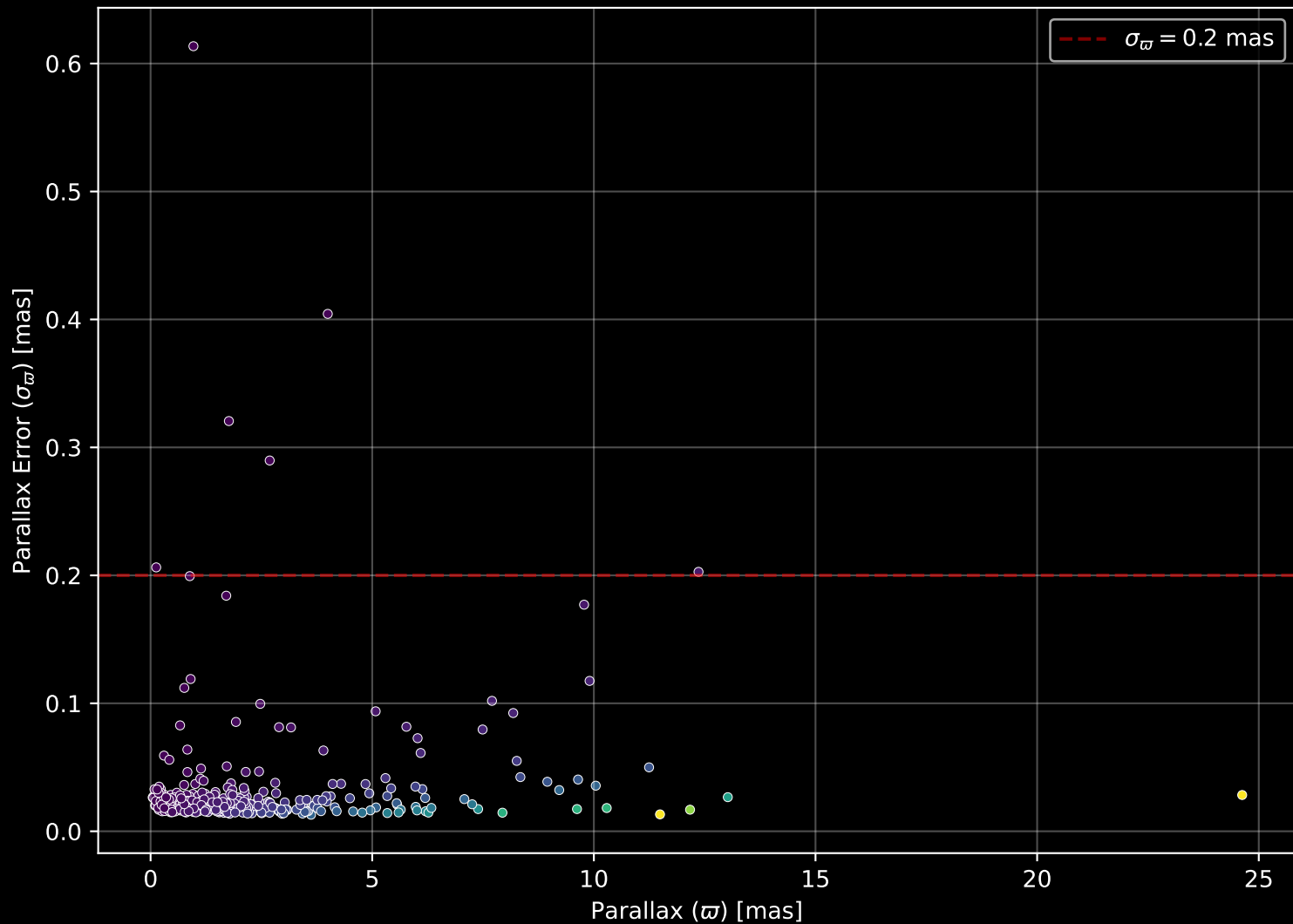
APOGEE DR17 Field: [179-25-O] Parallax Quality (n= 366)
