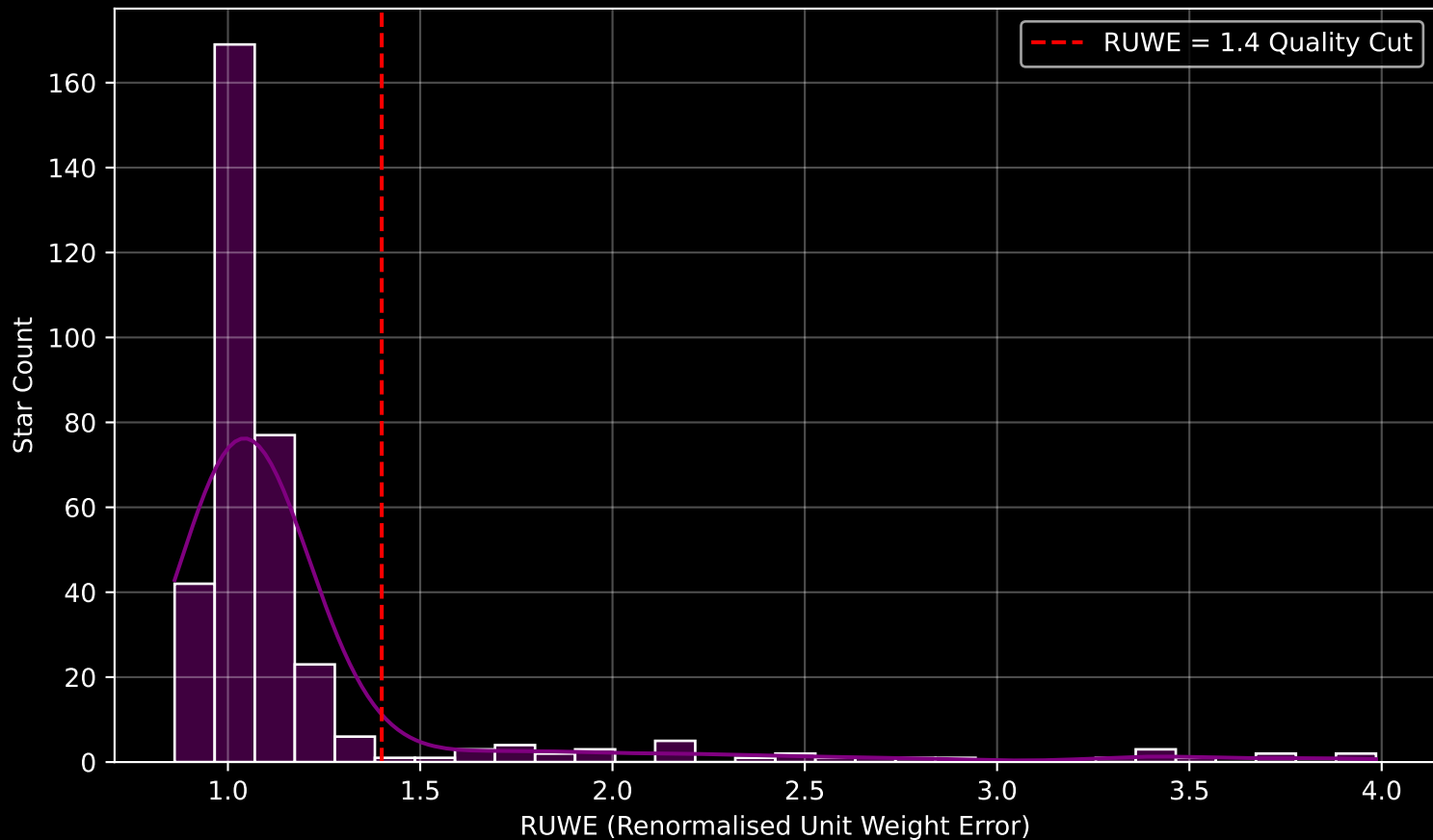
GAPOGEE DR17 Field [179-25-O] RUWE Distribution (n= 352)
