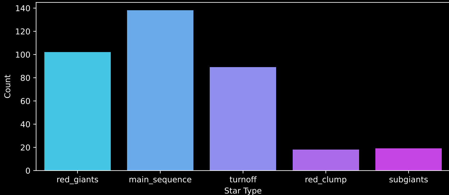
APOGEE DR17 Field: [179-25-O] Count plot of Star Type
