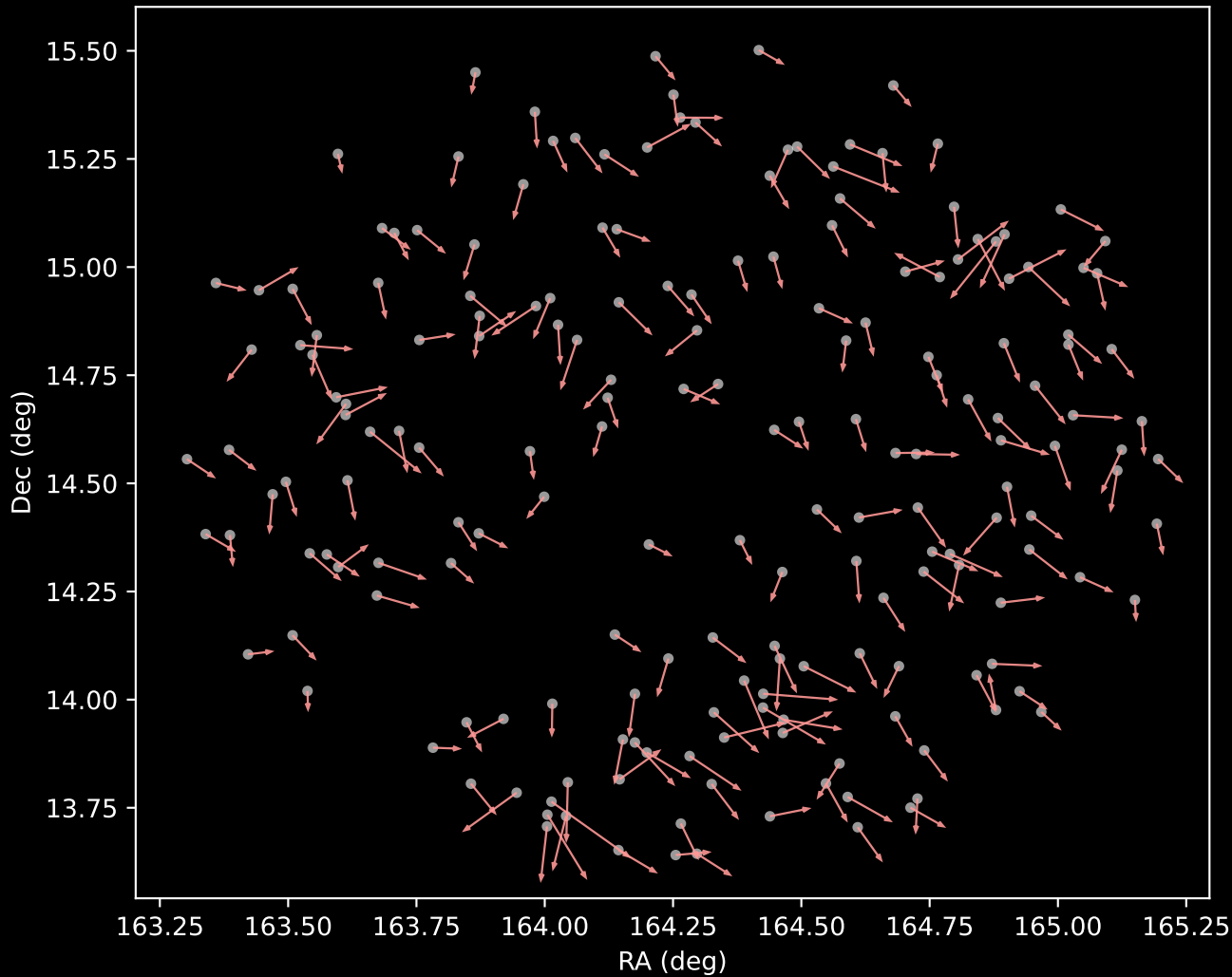
APOGEE DR17 Cluster 7 Proper Motion Vectors (n=191)
