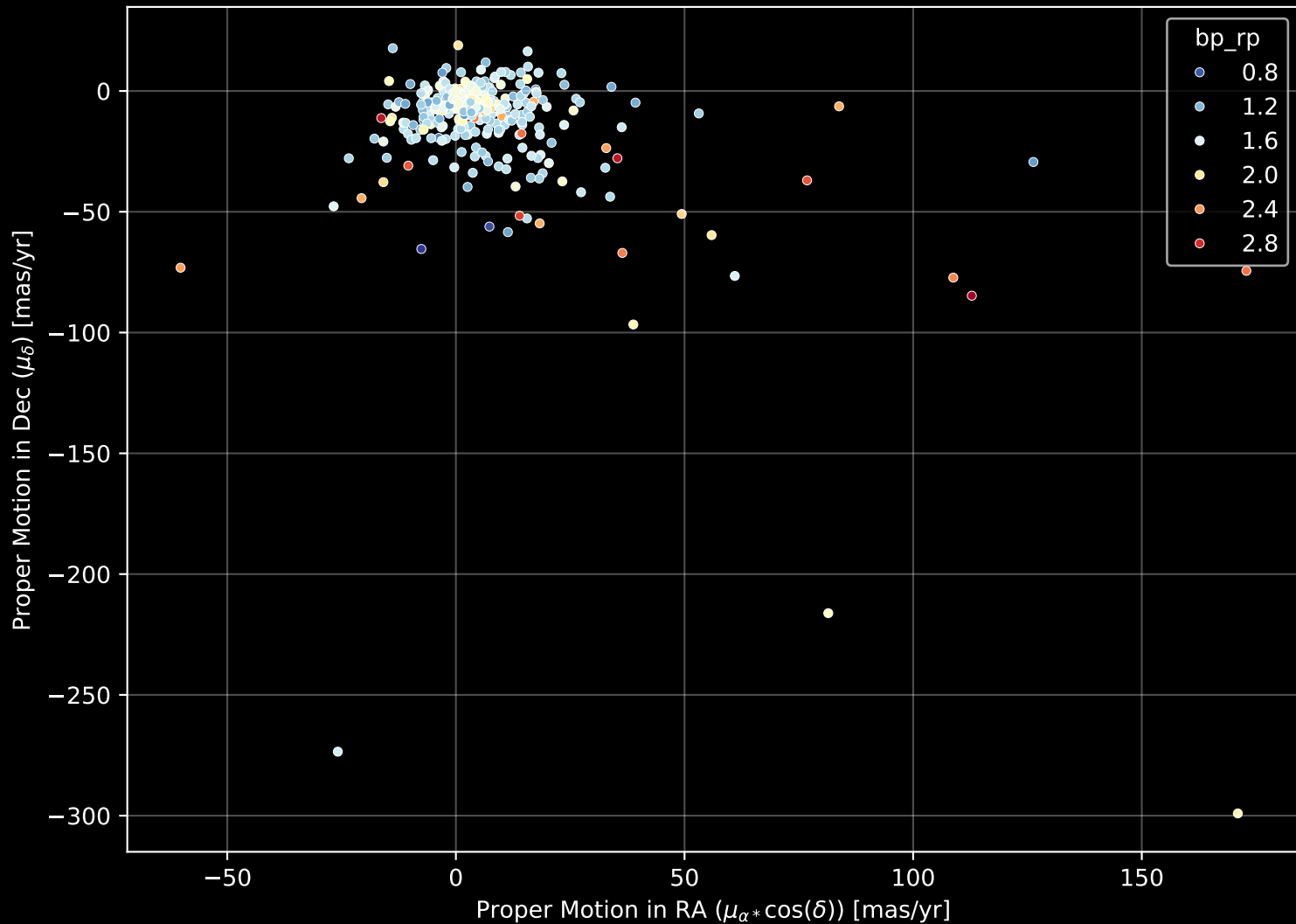
APOGEE DR17 Field: [179-25-O] Proper Motion Diagram (n= 366)
