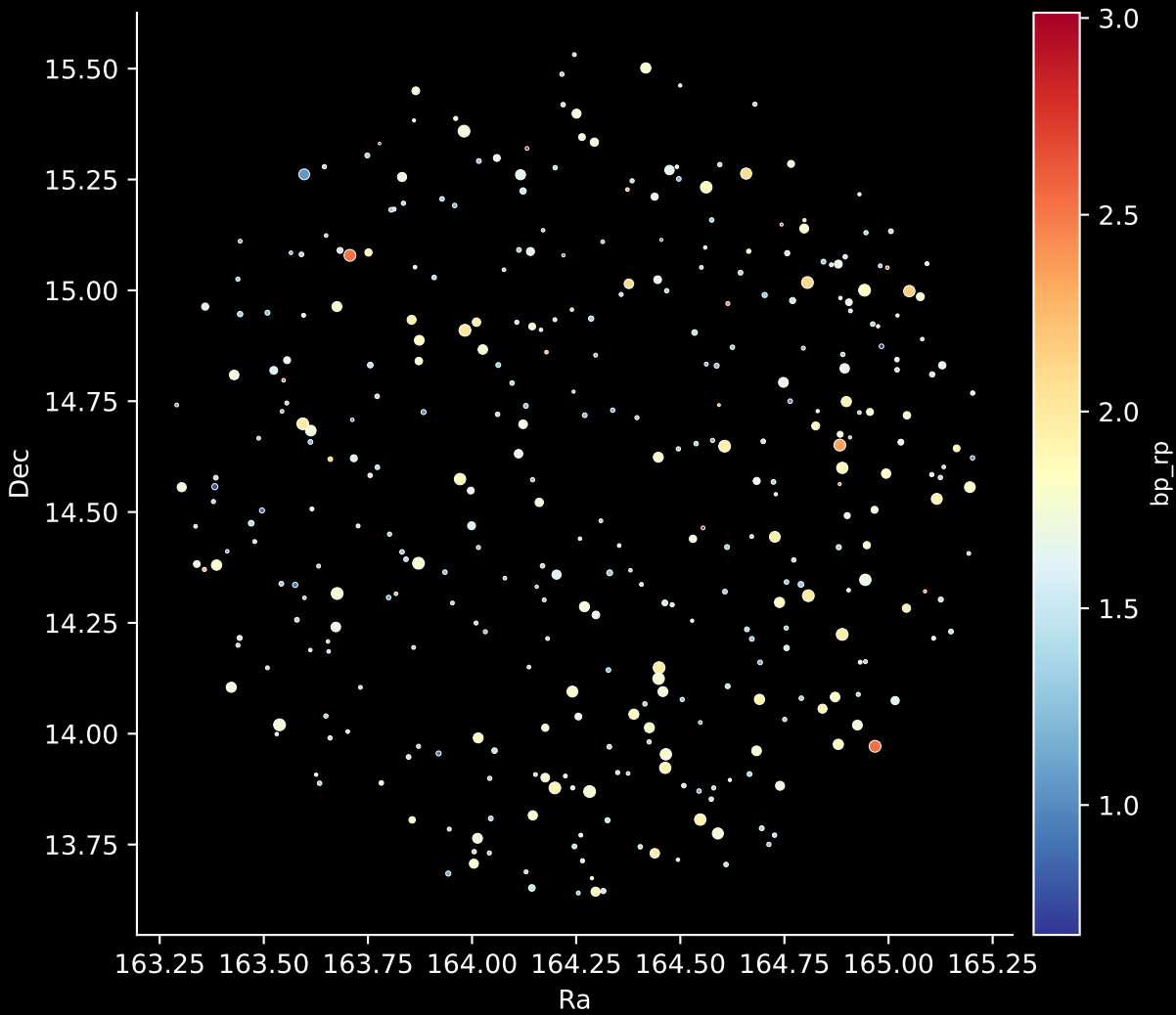
APOGEE DR17 Field: [179-25-O] Stars: 366
